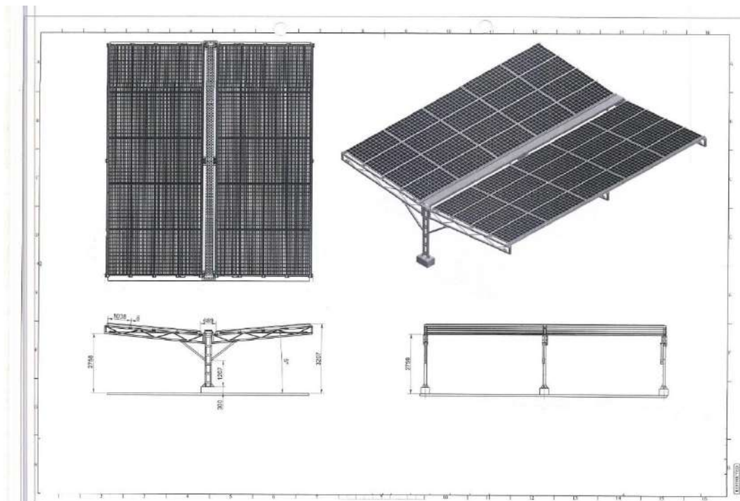
Figure A: Tentative Carport Structure Profile
